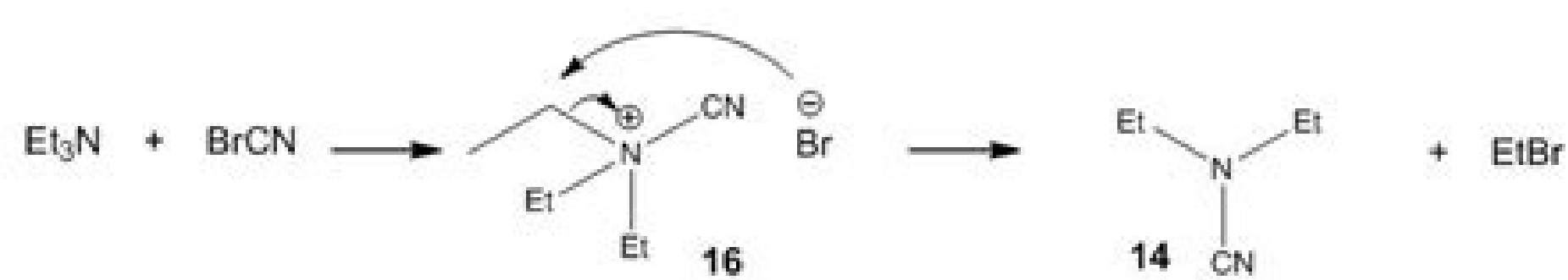
Scheme 8. Acyclic compounds reaction with cyanogen bromide.
