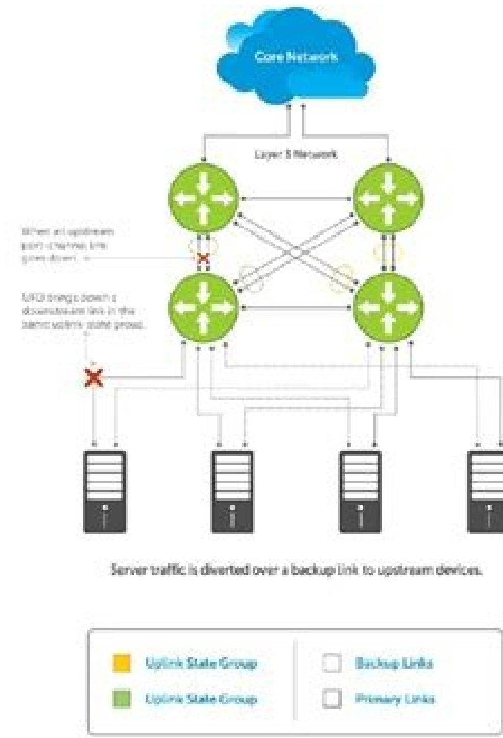
Figure 28. Uplink Failure Detection Example
